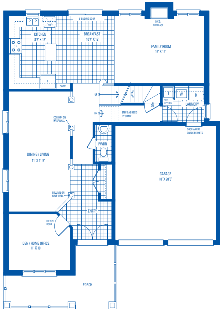
MAIN FLOOR Elevation A
