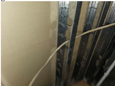
Pic. 37: Romex run thru metal studs without a grommet
