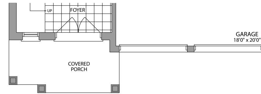
Ground Floor Elevation 2
