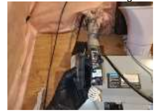
Pic. 28: ARCF breaker – removed and should be installed for safety
