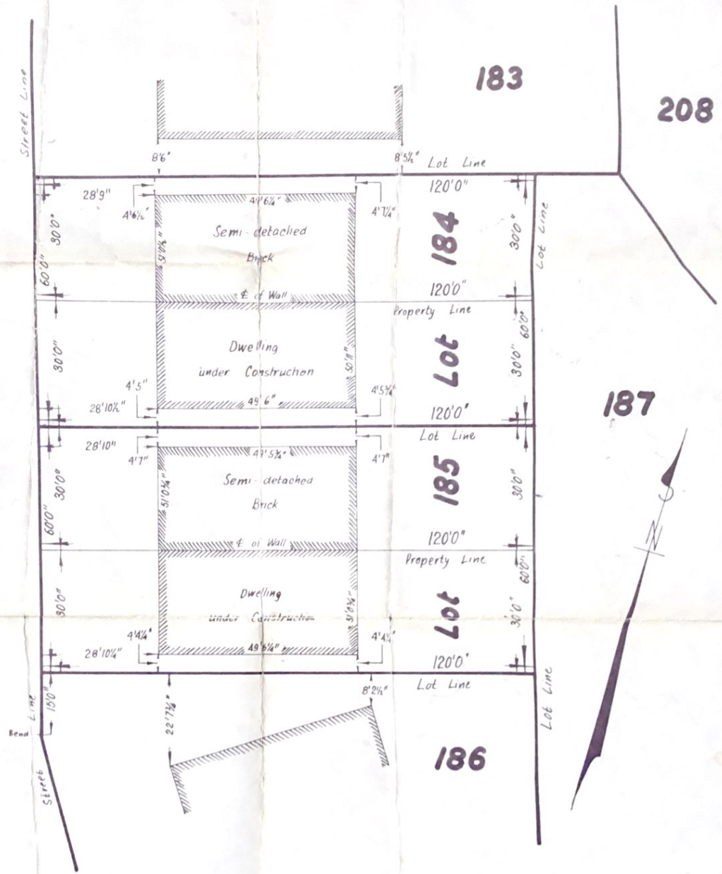
Plan showing LOTS 184 & 185 Reg'd Plan 5618 Township of North York - County of York Scale 1" = 25'
